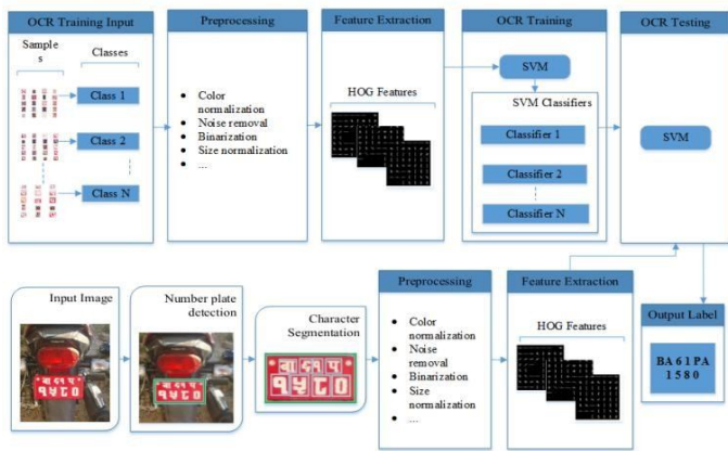
Fig. 3: Automatic license Plate Recognition System
