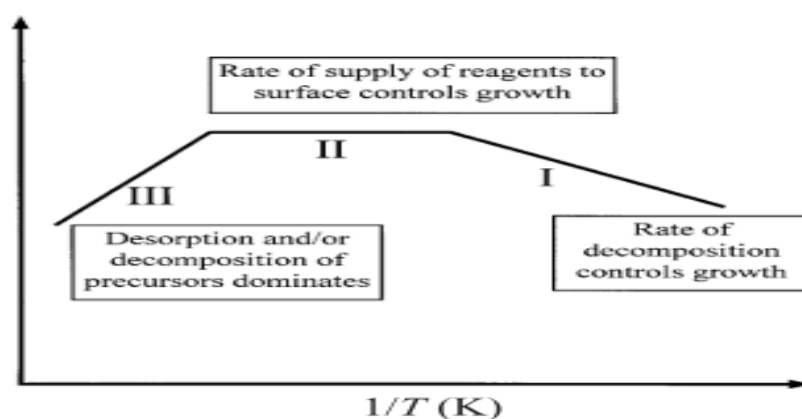
Figure 9: Temperature variation of a typical CVD process[18].
