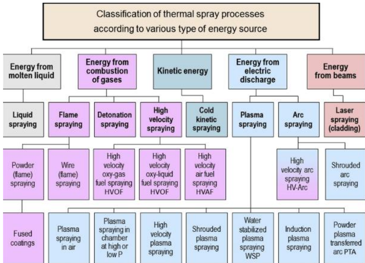
Figure 5 Classification of thermal spray process according to type of source energy
