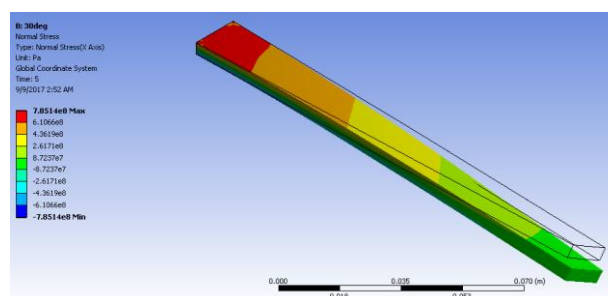
b) Cantilever beam with 30degree twist
