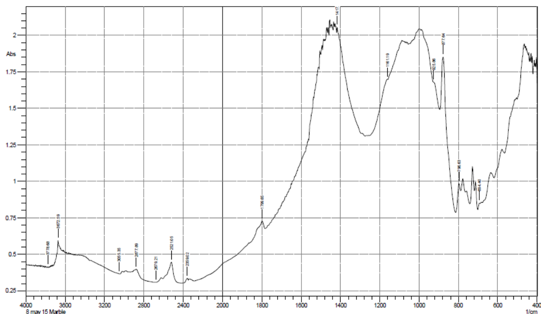
Figure 4.6: FTIR of waste marble dust
