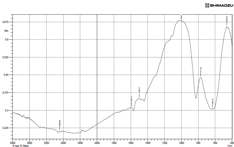
Figure 4.7: FTIR of waste crushed glass
