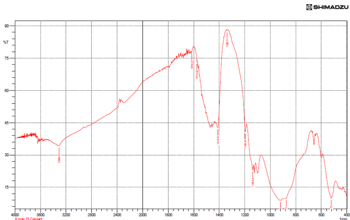
Figure 4.5: FTIR of OPC cement grade 43
