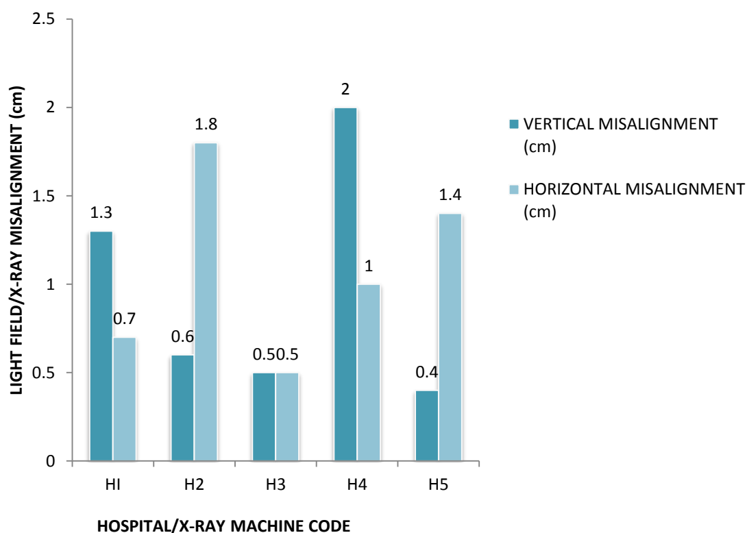
Figure 2: A Bar Chart Representing the Light Field/X-Ray beam Alignment Test Results on the 22.5 cm x 17.5 cm Collimator Light Field.
