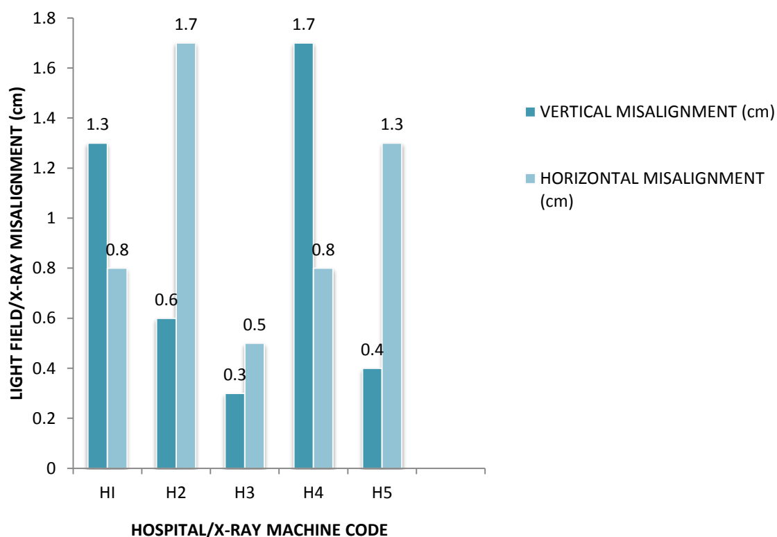
Figure1: A Bar Chart Representing the Light Field/X-Ray beam Alignment Test Results on the 12.5 cm x 12.5 cm Collimator Light Field.
