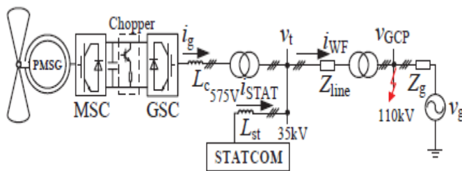
Fig .2. Structural Configuration of the PMSG based wind farm
