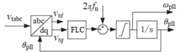
Fig .3. functional diagram of the phase locked loop
